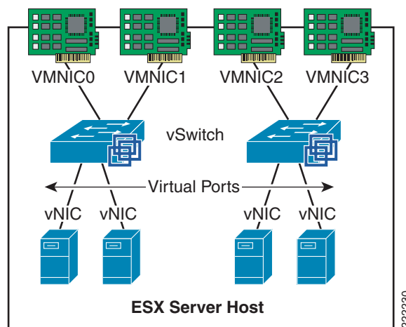
Figure 2 ESX Server Interfaces
