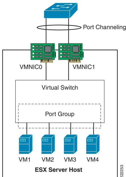
Figure 13 vSwitch EtherChanneling
