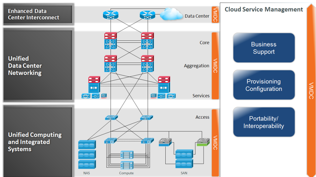
Figure 1 VMDC Reference Architecture
