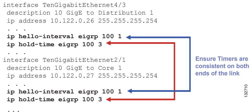
Figure 11 Reducing EIGRP Hello and Dead Timers
