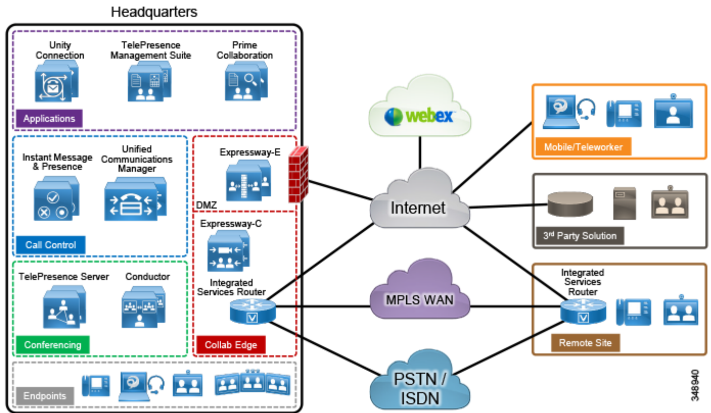
Figure 1-1 Cisco Preferred Architecture for Enterprise Collaboration
