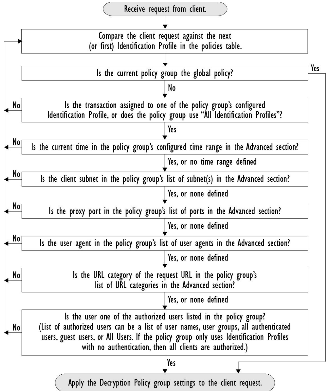
Figure 2: Policy Group Transaction Flow for Decryption Policies
