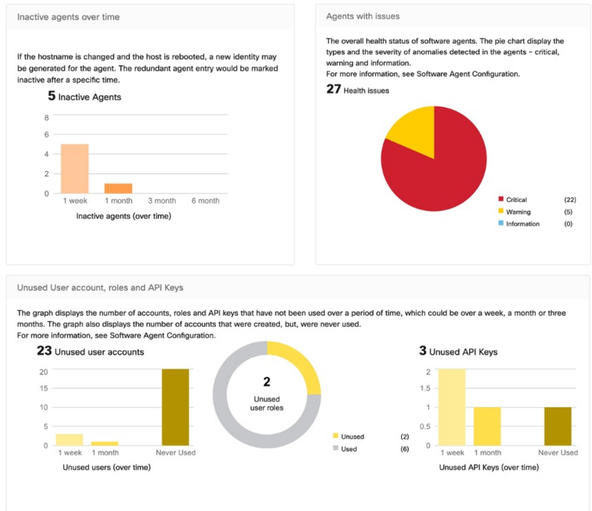
Figure 6: Workload Summary
