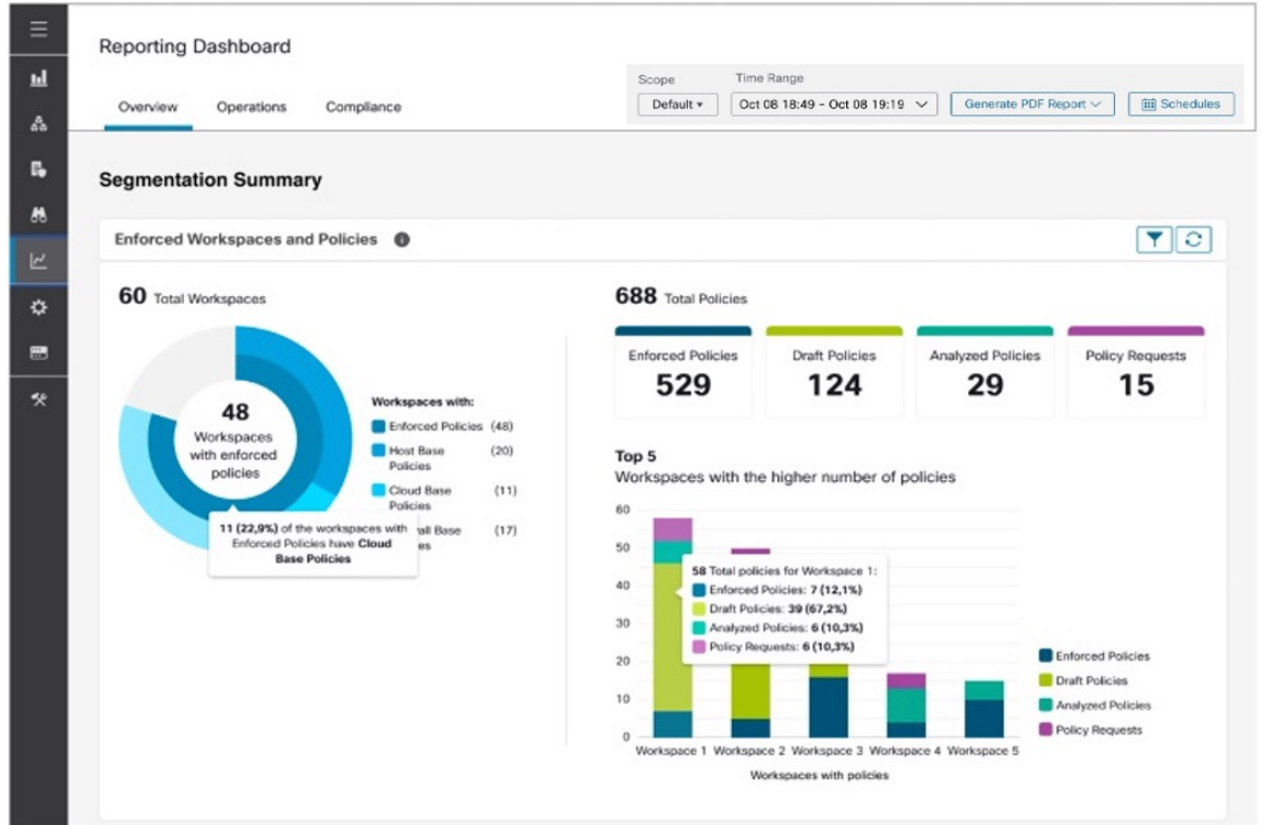
Figure 1: Segmentation Summary
