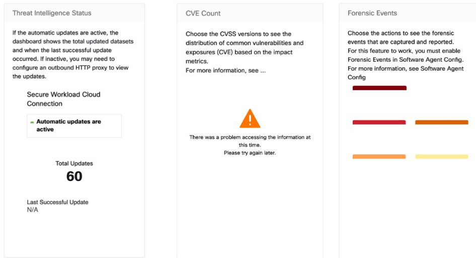
Figure 5: Security Summary
