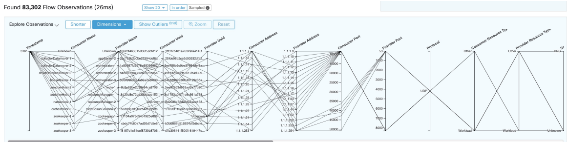
Figure 15: Explore Observations
