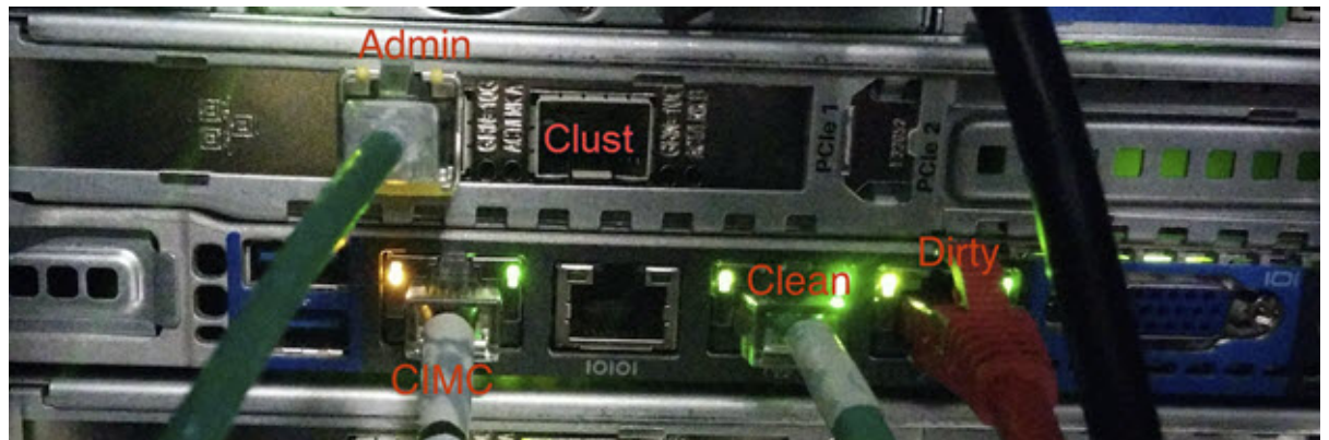
Figure 25: Clust Interface Setup for Cisco UCS M4 C220
