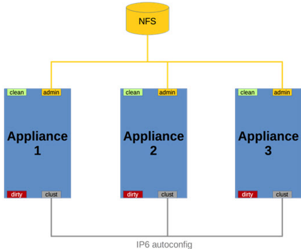
Figure 24: Clustering Network Diagram
