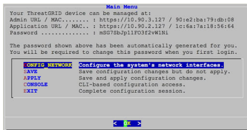
Figure 2: TGSN Dialog (Connected to a Network Configured to Use DHCP)
