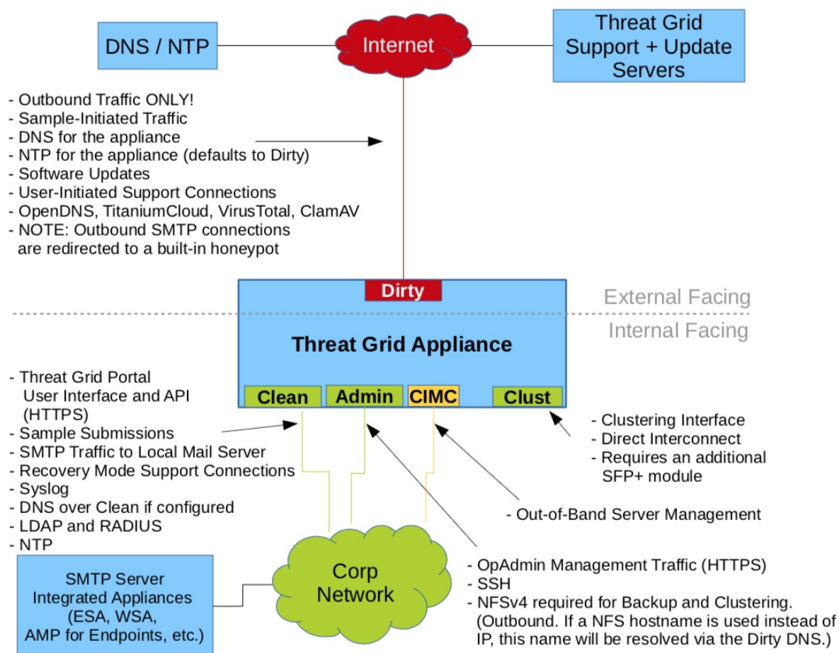
Figure 3: Network Interfaces Setup Diagram
