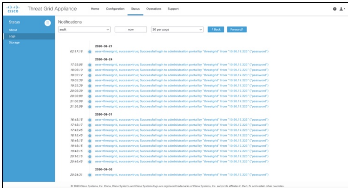
Figure 2: Notifications
