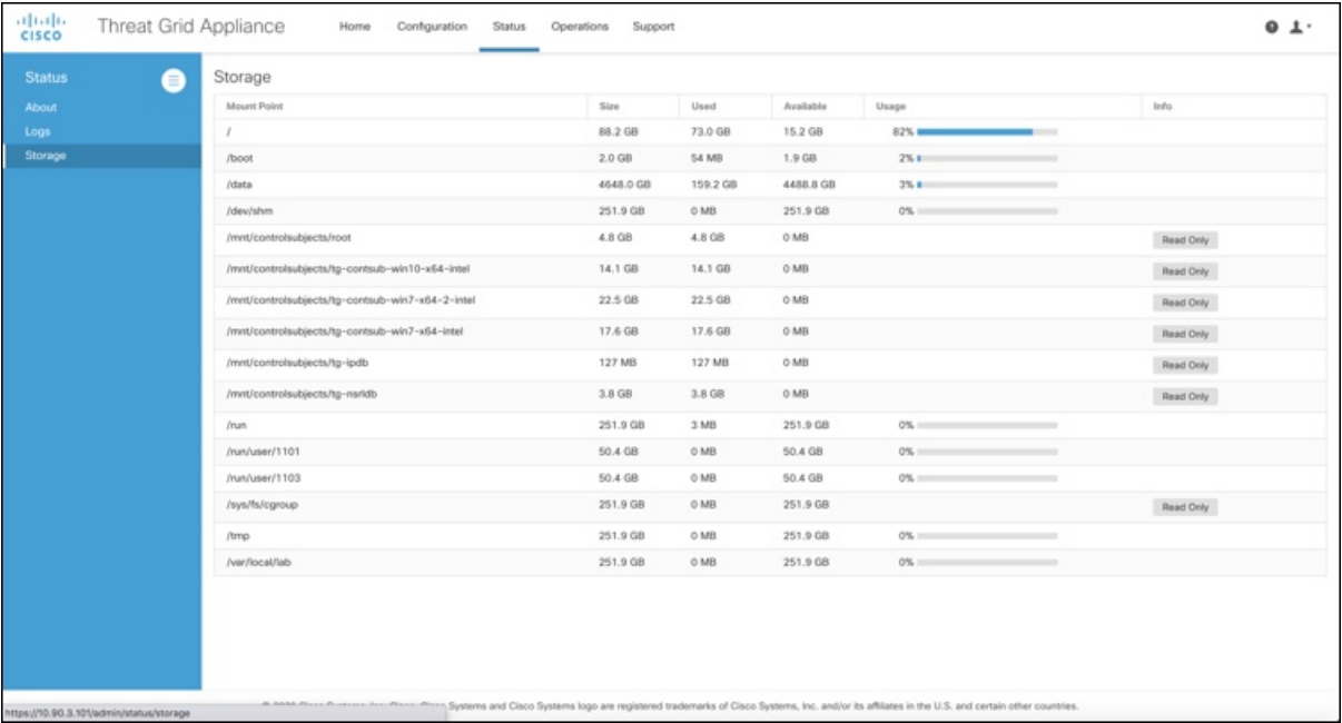
Figure 3: Storage
