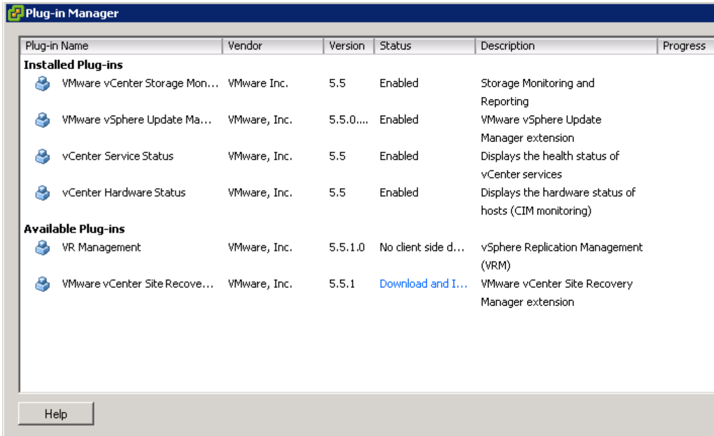
Figure 8: Plug-in Manager
