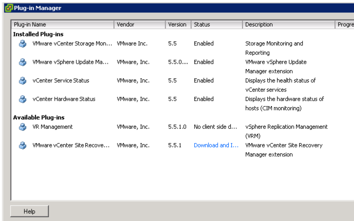
Figure 4: Plug-in Manager
