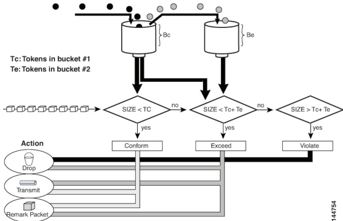
Figure 3: Two-Token Bucket Algorithm
