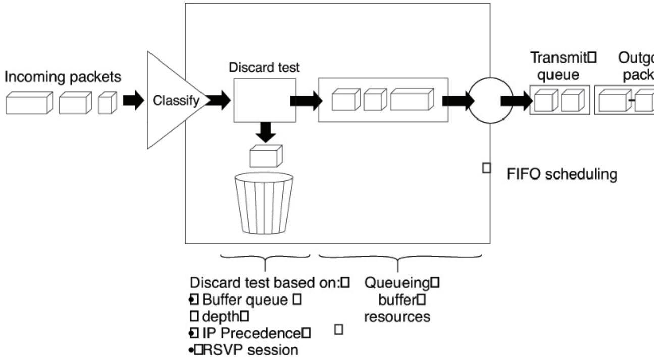
Figure 1: Weighted Random Early Detection
