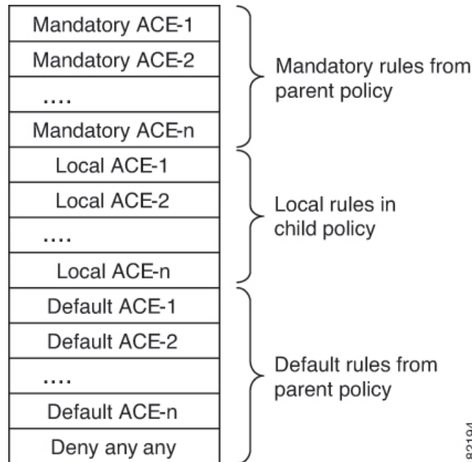
Figure 2: Order of Rules When Using Inheritance
