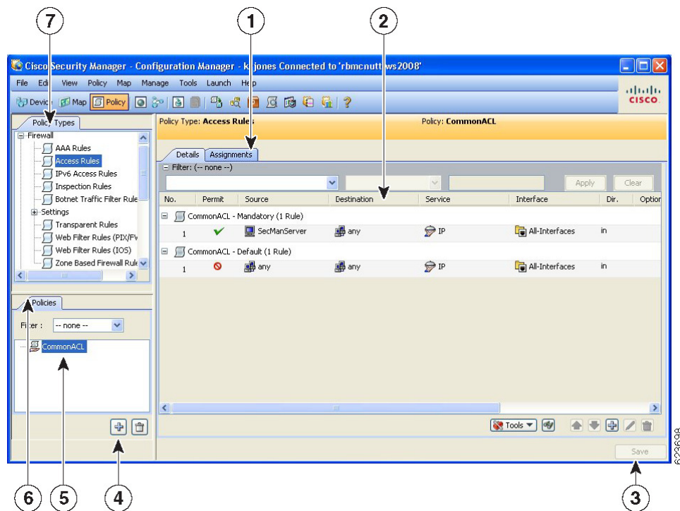
Figure 3: Policy View
