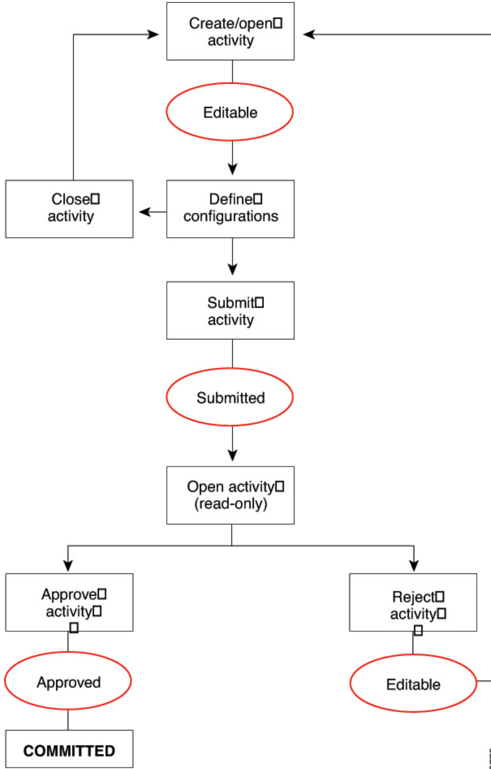
Figure 3: Activity Workflow with an Approver
