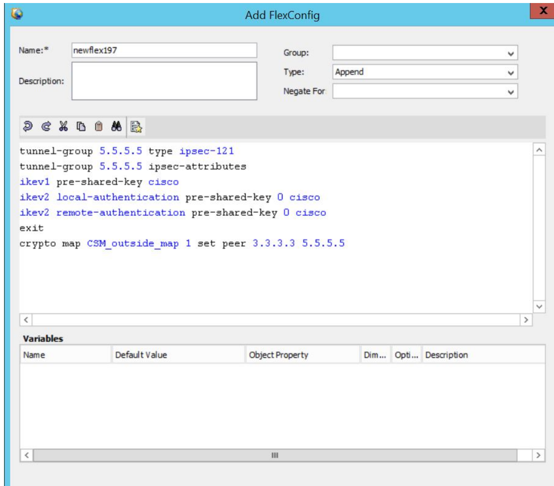
Figure 4: Multi Peer-Specific and Tunnel-Group CLI
