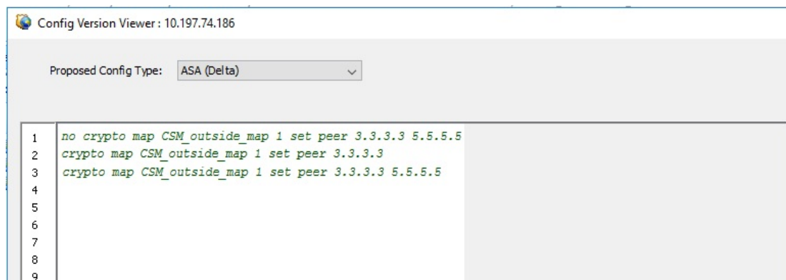
Figure 5: CLI Negation
