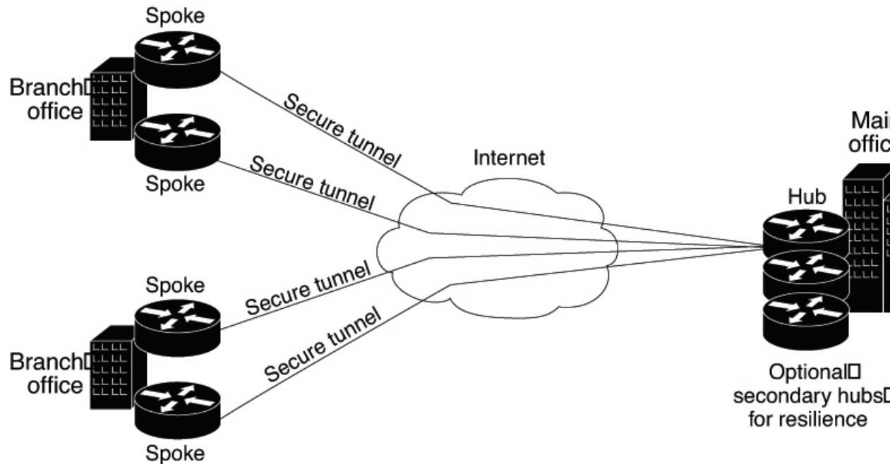
Figure 1: Hub-and-spoke VPN Topology
