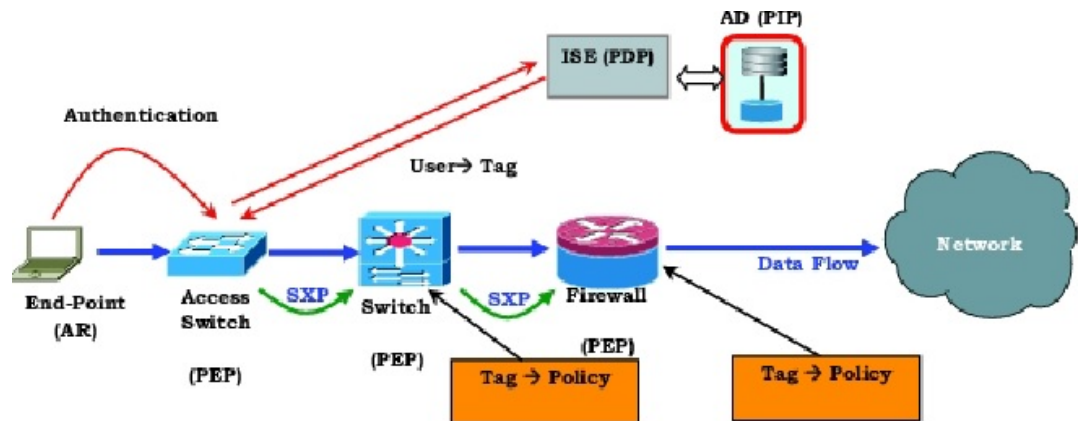
Figure 2: Security Policy Enforcement
