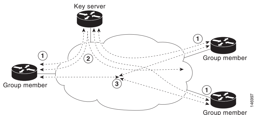
Figure 29-1 General GET VPN Operation
