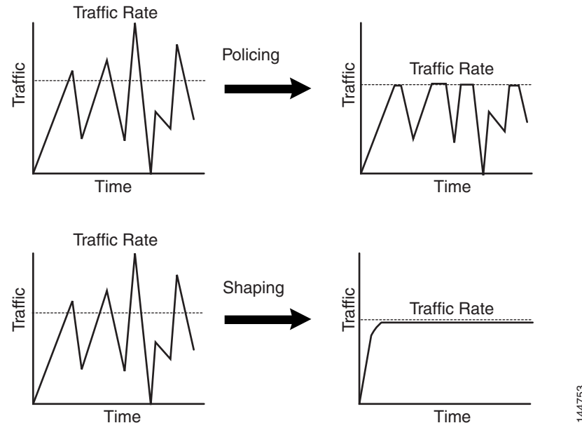
Figure 66-2 Traffic Policing vs. Traffic Shaping
