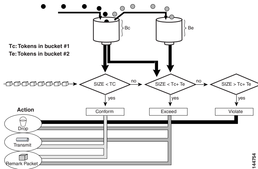
Figure 66-3 Two-Token Bucket Algorithm
