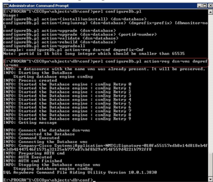
Figure 1 Re-registering Database Parameters
