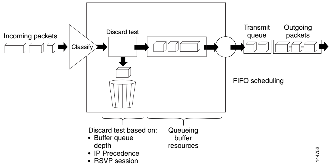
Figure 65-1 Weighted Random Early Detection
