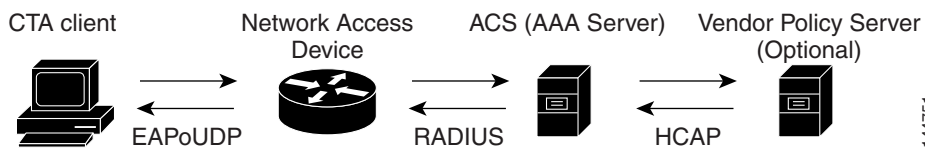
Figure 63-2 NAC System Flow
