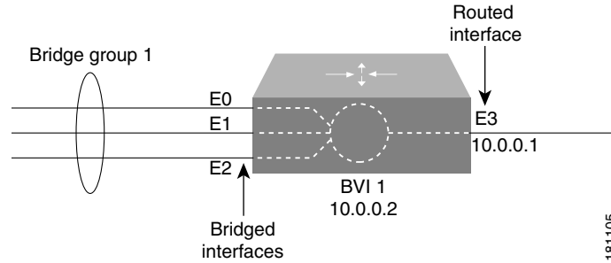
Figure 59-2 Bridge-Group Virtual Interface
