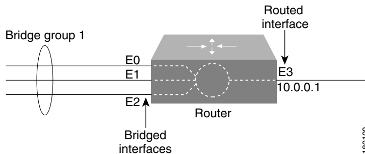
Figure 59-1 Transparent Bridging
