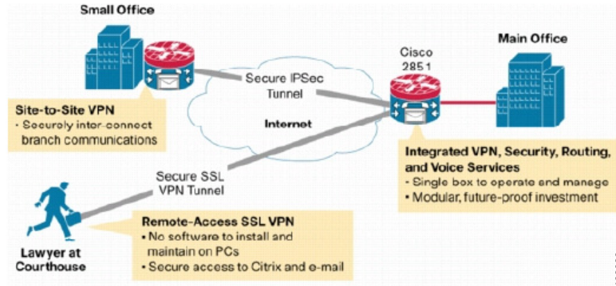
Figure 28-1 Secure SSL VPN Access Example
