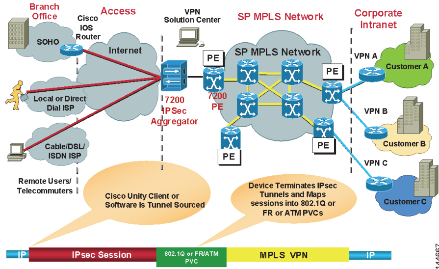
Figure 1-5 VRF-Aware IPsec Two-Box Solution
