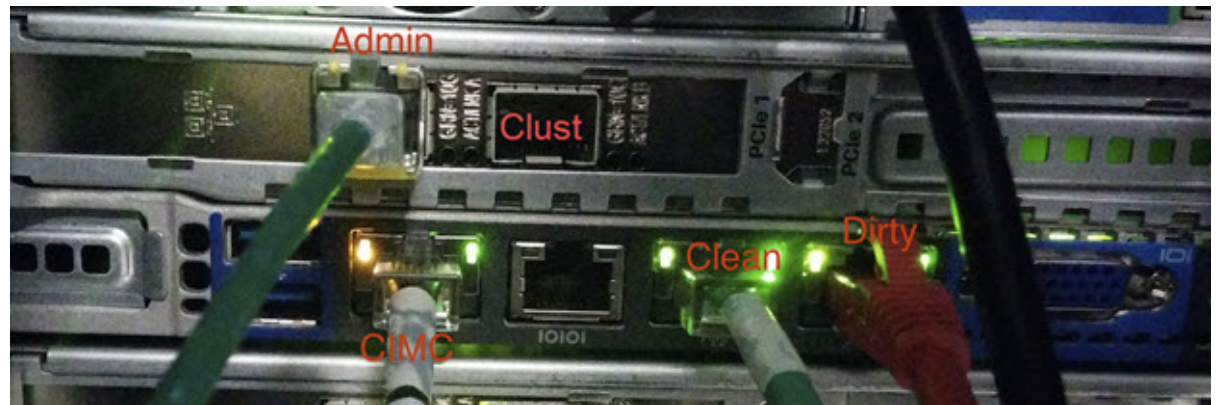
Figure 51: Clust Interface Setup for Cisco UCS M4 C220
