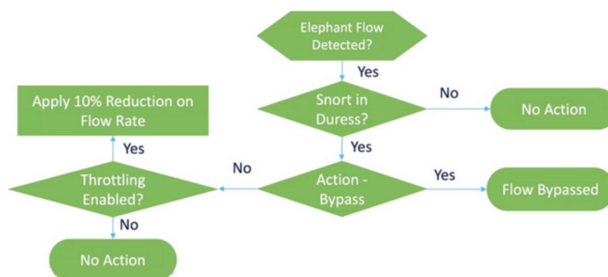
Figure 4: Elephant Flow Workflow
