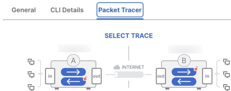
Figure 4: Packet Tracer
