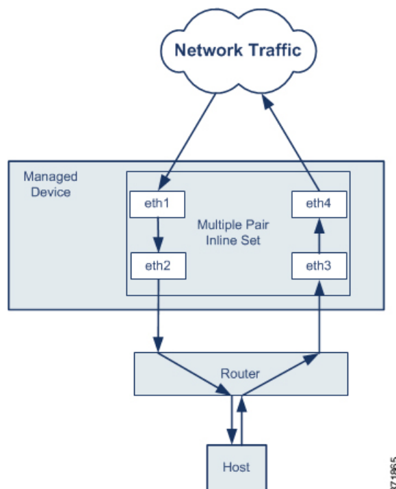
Figure 1: Asynchronous Routing
