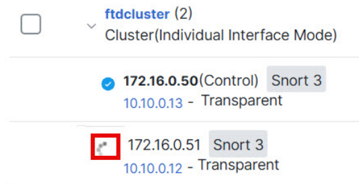
Figure 15: Node Registration
