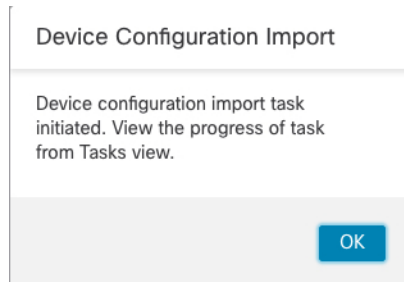
Figure 16: Acknowledge Import
