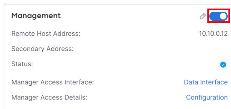
Figure 34: Disable Management
