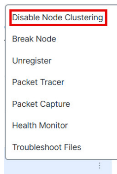
Figure 20: Disable Clustering
