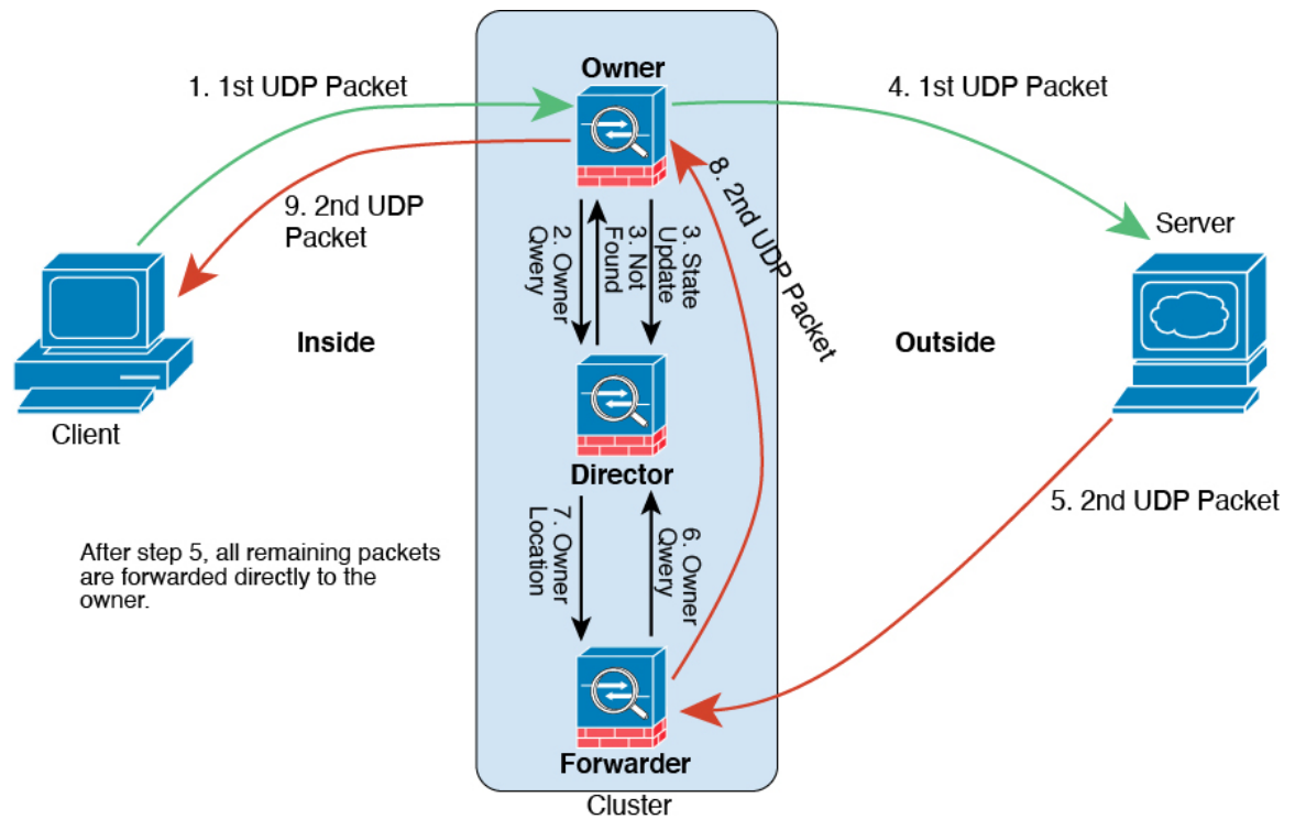
1. Figure 33: ICMP and UDP Data Flow
