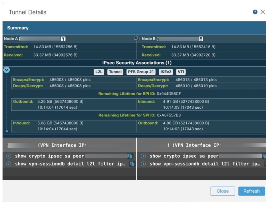
Figure 1: Tunnel Status &gt; View &gt; CLI Details
