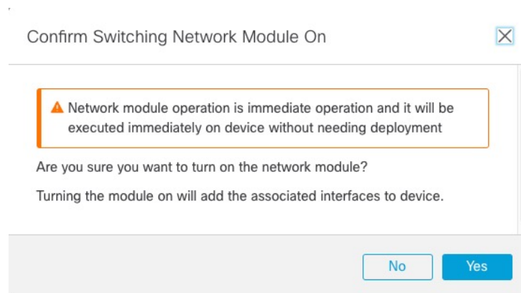
Figure 30: Confirm Enable
