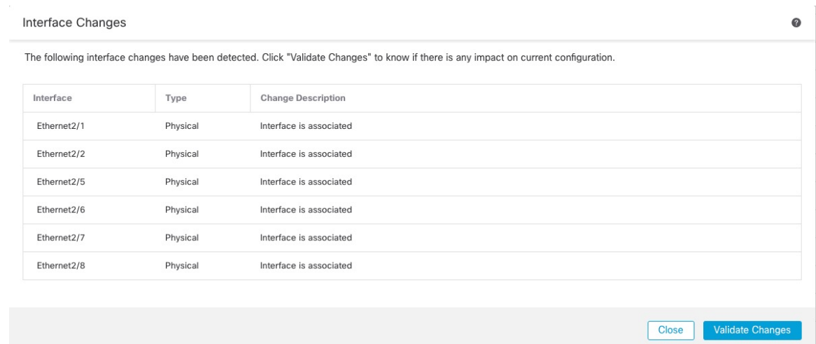
Figure 20: Interface Changes
