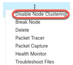
Figure 21: Disable Clustering
