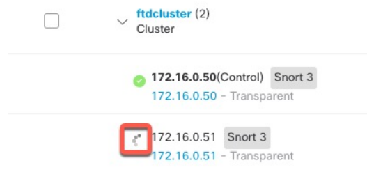
Figure 16: Node Registration
