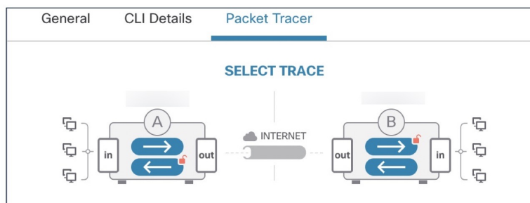
Figure 1: Packet Tracer
