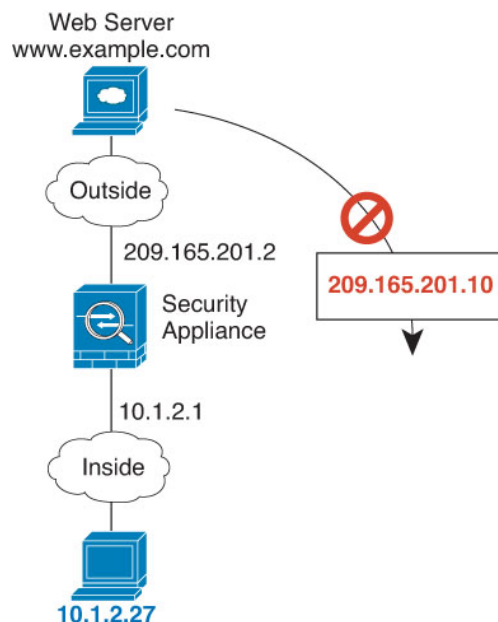
Figure 5: Remote Host Attempts to Initiate a Connection to a Mapped Address
