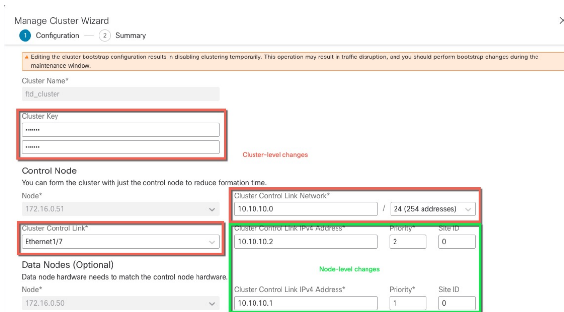
Figure 23: Manage Cluster Wizard
