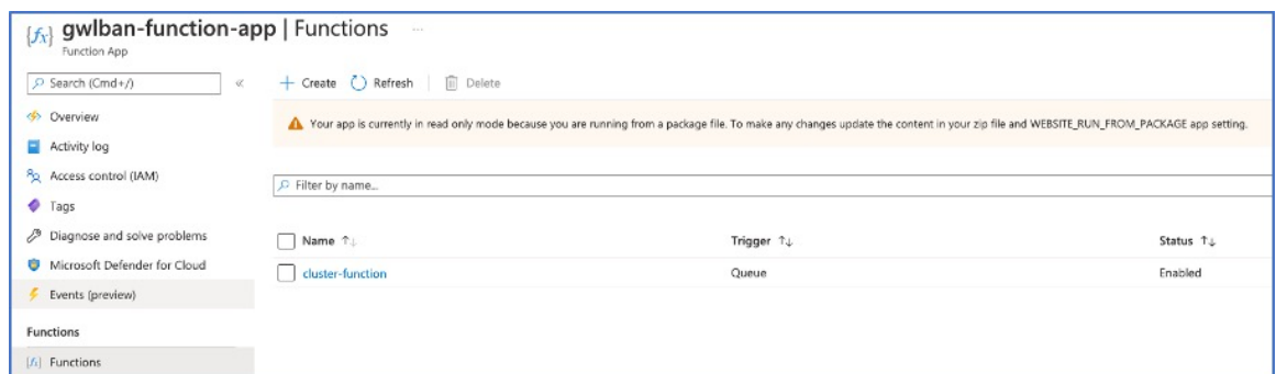
Figure 11: Functions
