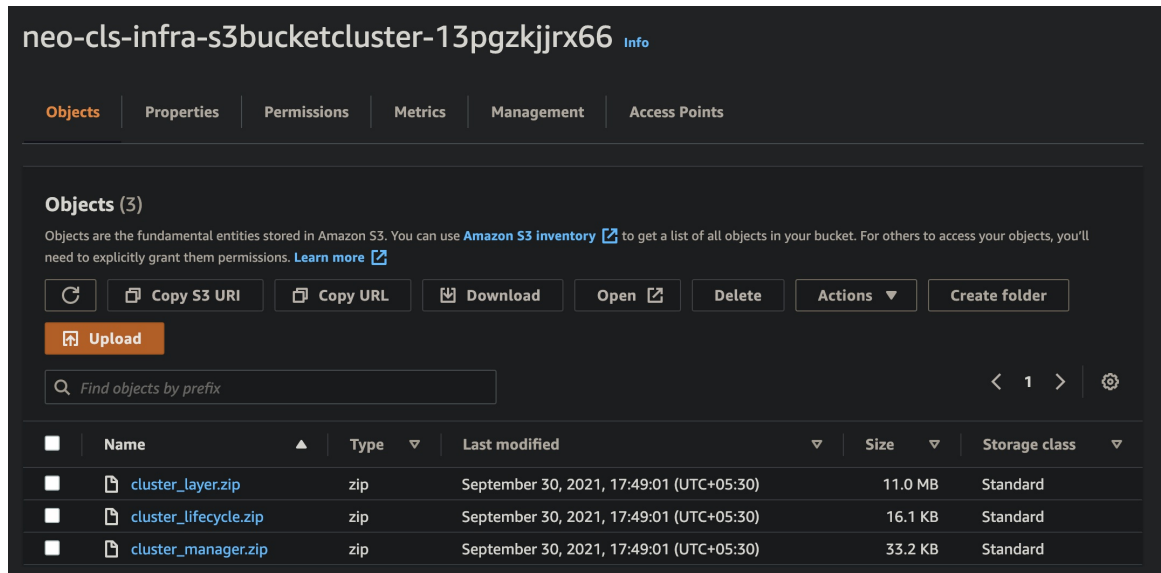
Figure 3: S3 Bucket
