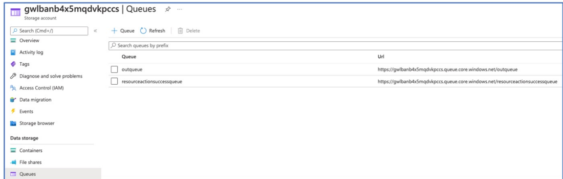
Figure 13: Outqueue
