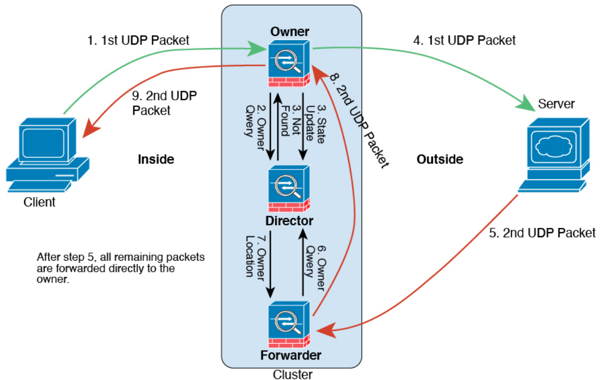
1. Figure 12: ICMP and UDP Data Flow
