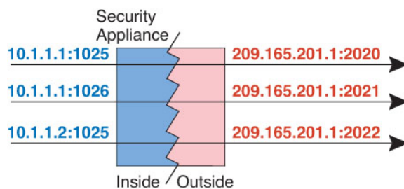
Figure 6: Dynamic PAT
