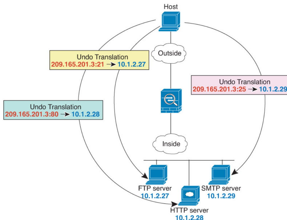
Figure 17: Static NAT-with-Port-Translation
