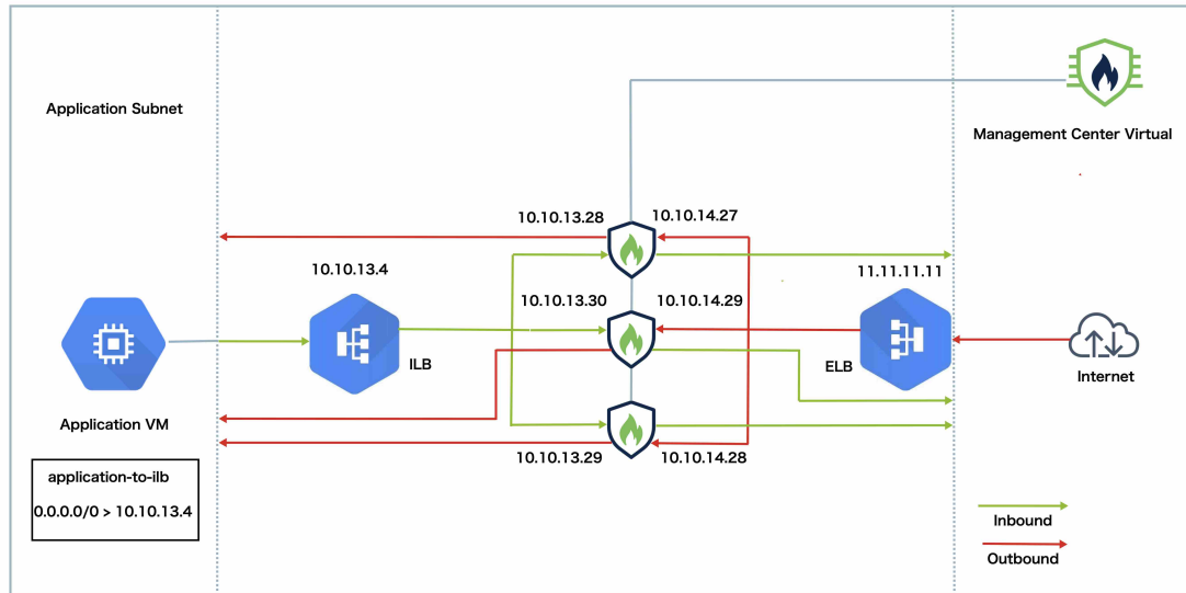
Figure 19: Sample Topology
