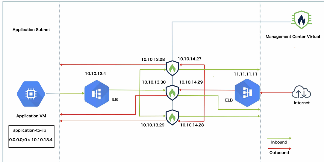
Figure 20: Sample Topology
