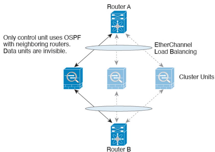
Figure 16: Dynamic Routing
