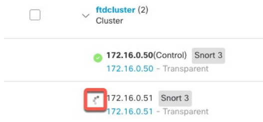
Figure 18: Node Registration
