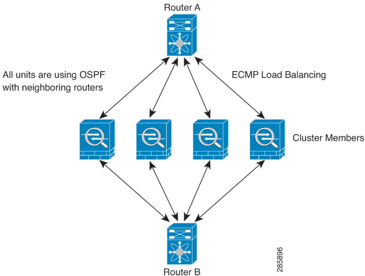
Figure 15: Dynamic Routing in Individual Interface Mode
