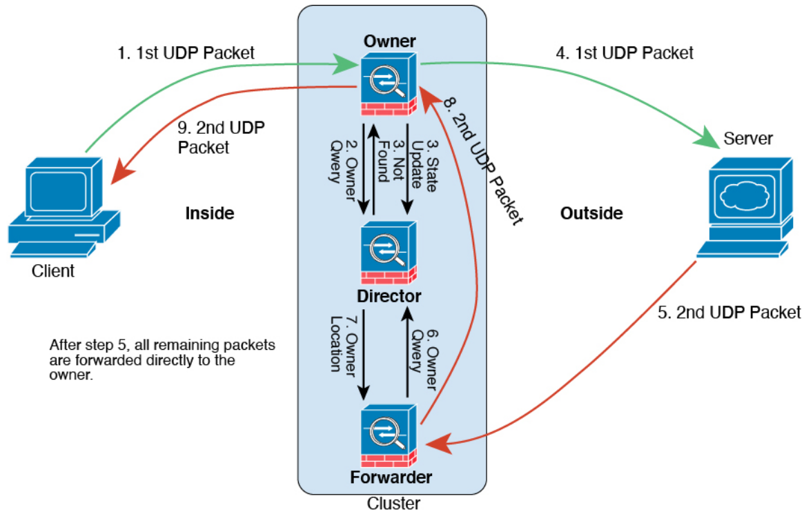
1. Figure 16: ICMP and UDP Data Flow
