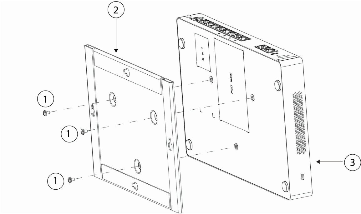
Figure 3: Attach the Wall-Mount Bracket to the Chassis
