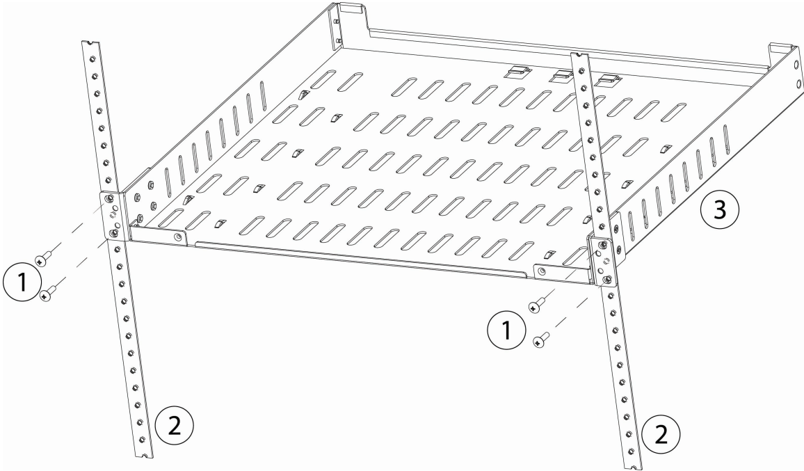
Figure 5: Install the Rack Shelf into the Rack
