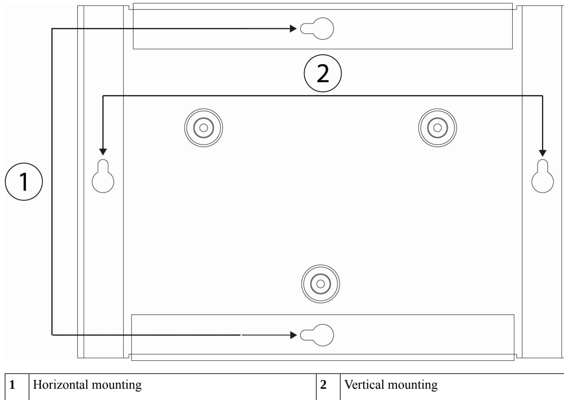
Figure 2: Wall-Mount Bracket
