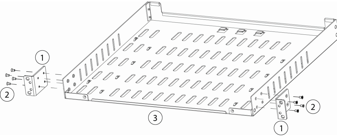
Figure 4: Install the Rack-Mount Brackets onto the Rack Shelf
