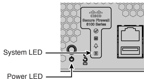
Figure 2: LEDs
