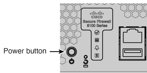
Figure 1: Power button
