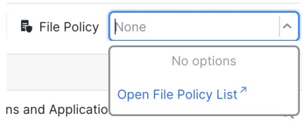
Figure 32: File Policy
