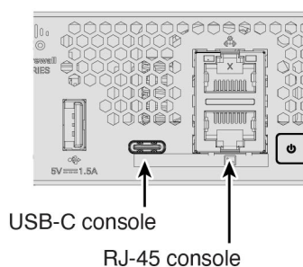
Figure 5: Console Port
